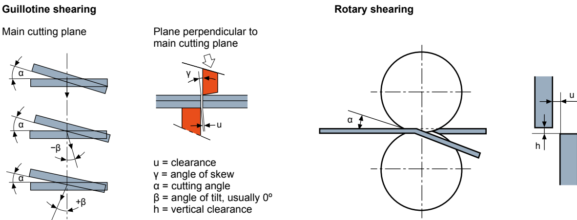
Figure 2. Mechanical cutting processes
