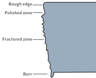
Figure 3. Parts of the shear face
