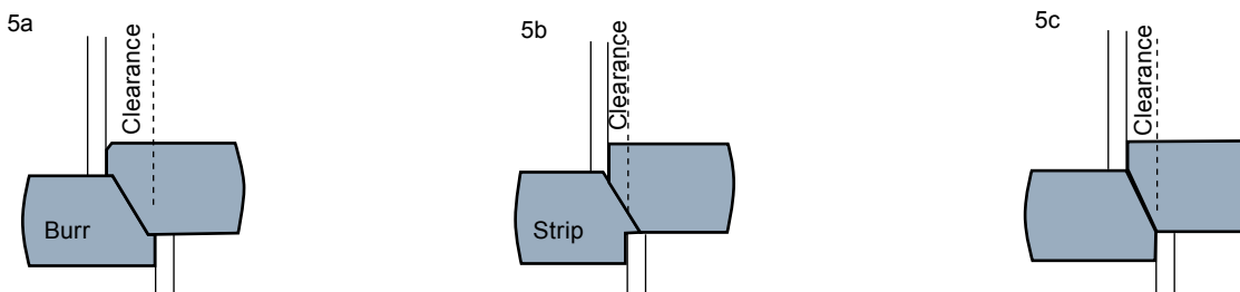
Figure 5. Affect of clearance ( u ) on cutting
