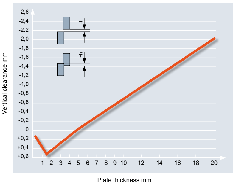
Figure 6. Rotary shearing. Recommended vertical clearance (h) values
